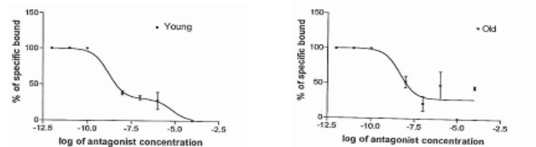
Fig. 2. Non linear regression curve for [ 3 H] Norepinephrine vs Prazosin in pancreatic islets
