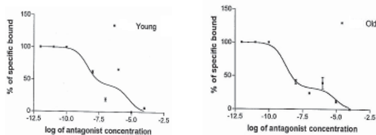
Fig.3. Non linear regression curve for [ 3 H] Norepinephrine vs Atenolol in pancreatic islets
